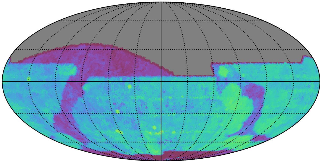
baseline_v3.0_10yrs All sky i band: Median Season Length
