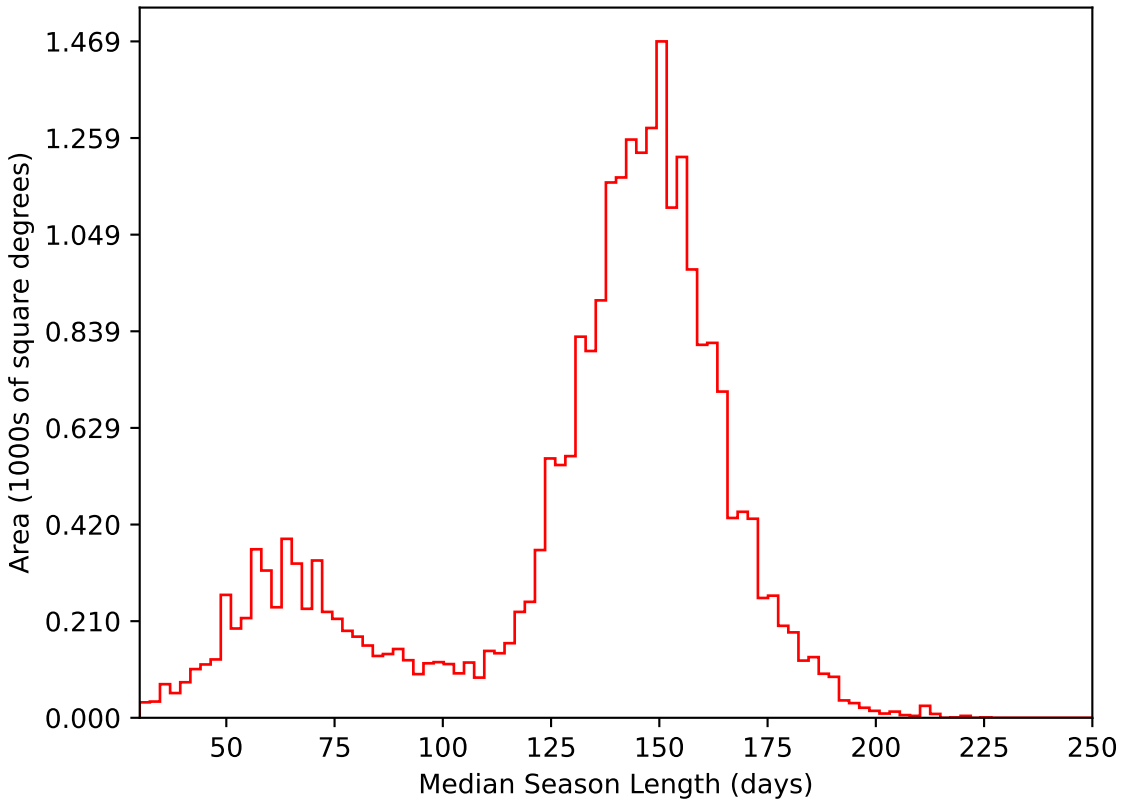
baseline_v3.0_10yrs All sky i band: Median Season Length
