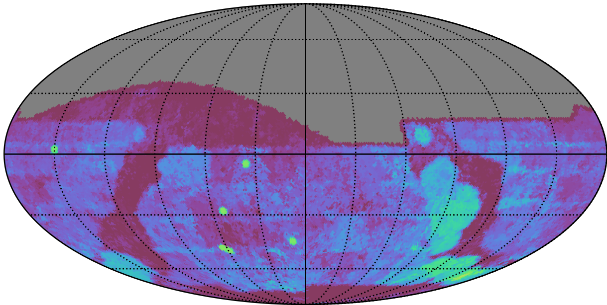
baseline_v3.0_10yrs All sky g band: Median Season Length
