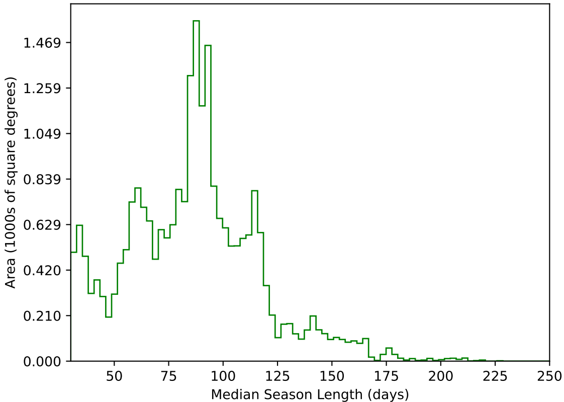
baseline_v3.0_10yrs All sky g band: Median Season Length
