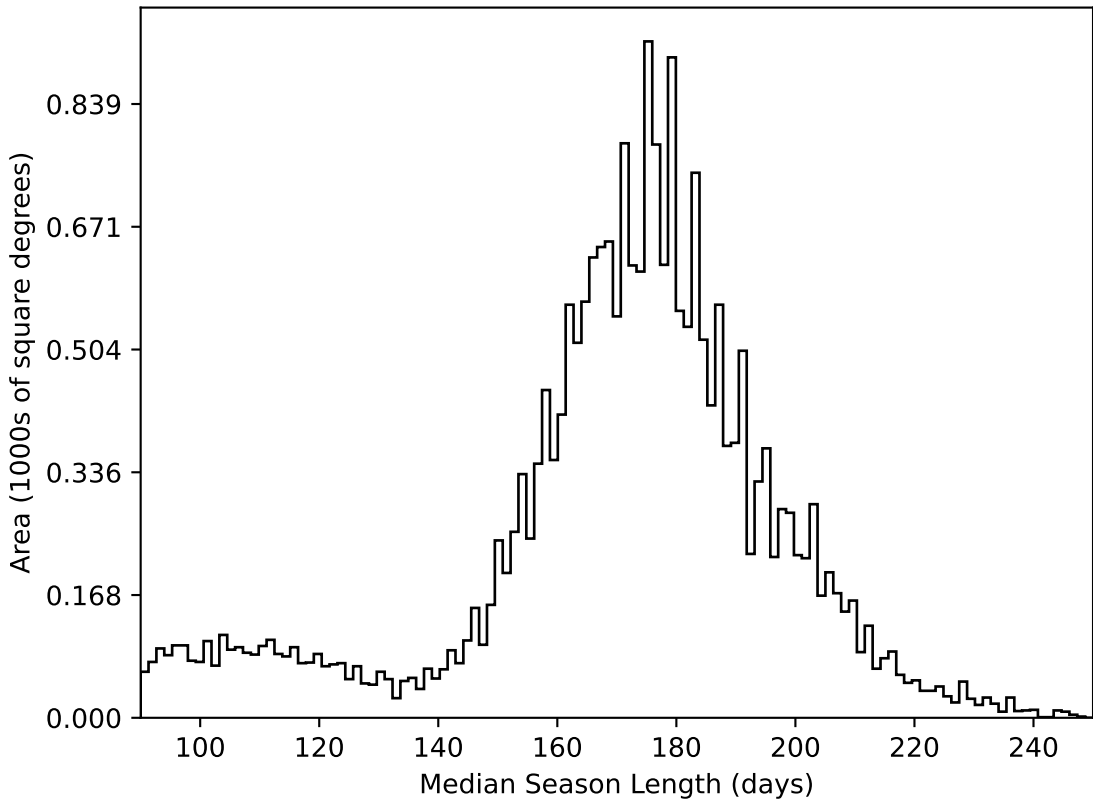
baseline_v3.0_10yrs All sky all bands: Median Season Length
