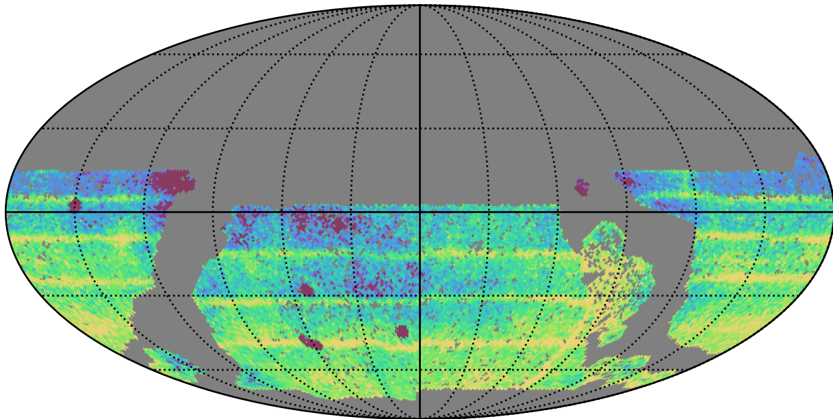
baseline_v3.0_10yrs WFD: Median Intra-Night Gap
