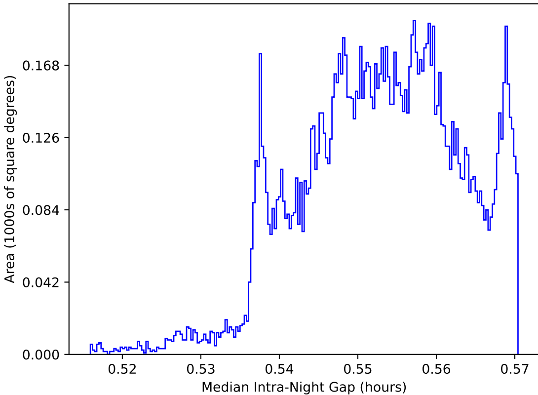
baseline_v3.0_10yrs WFD: Median Intra-Night Gap
