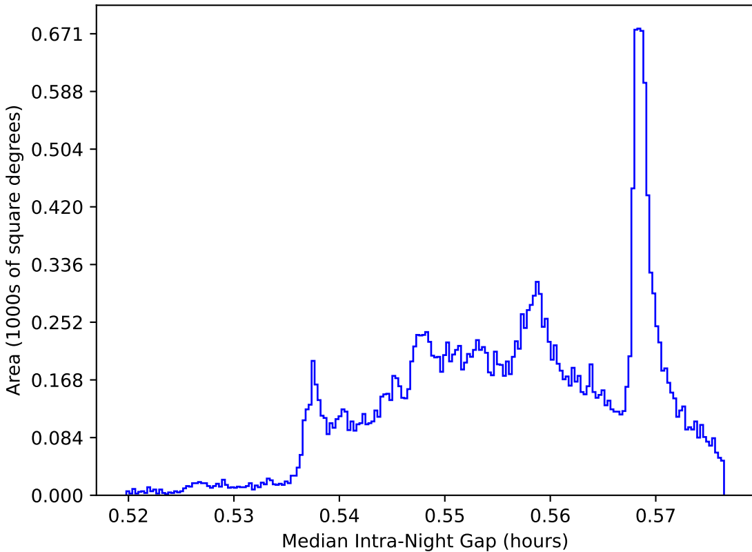
baseline_v3.0_10yrs All sky: Median Intra-Night Gap
