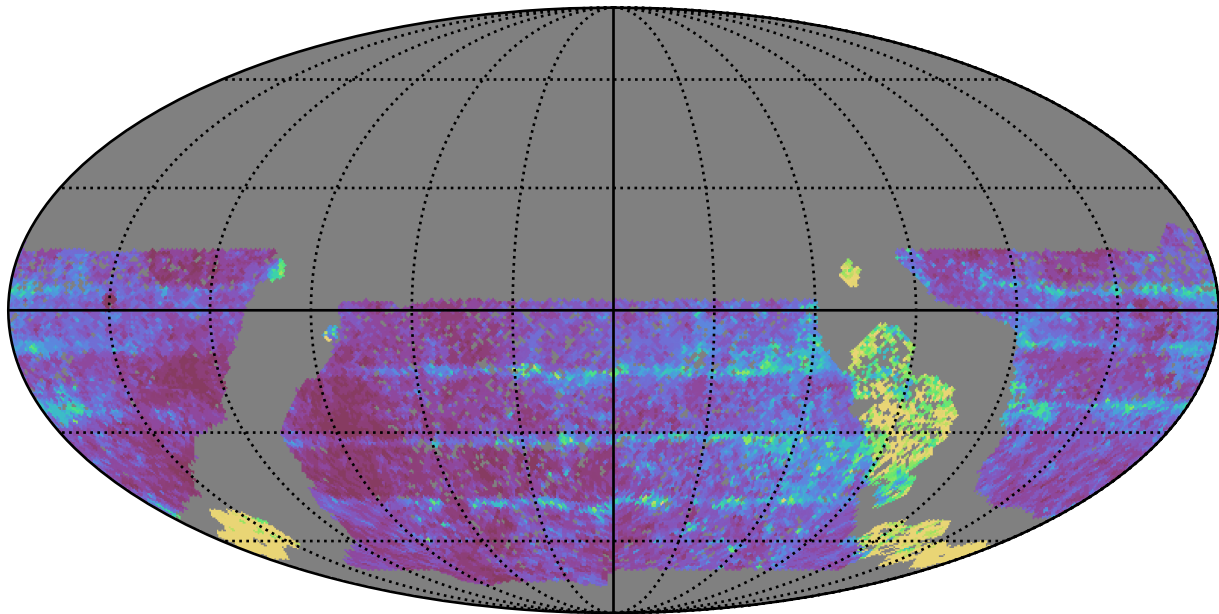
baseline_v3.0_10yrs WFD z band: Median Inter-Night Gap
