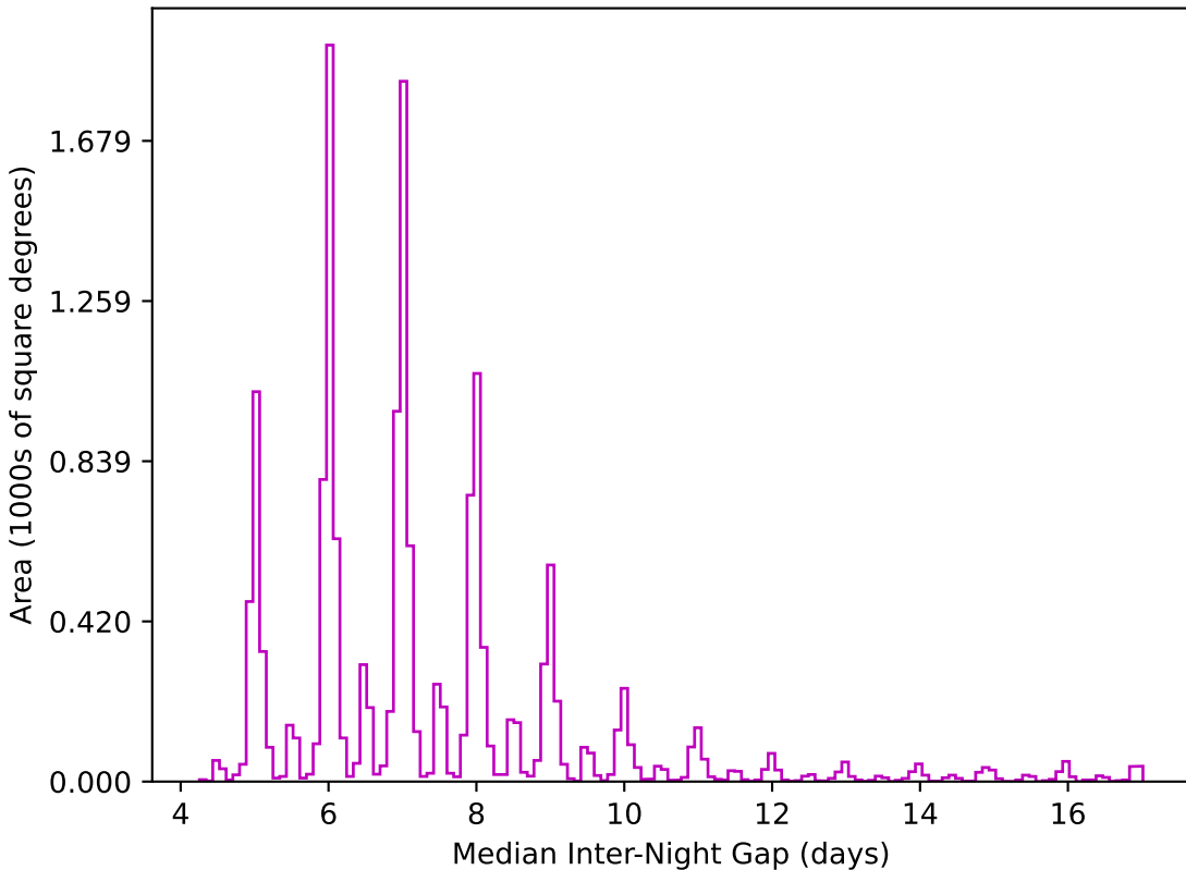
baseline_v3.0_10yrs WFD z band: Median Inter-Night Gap
