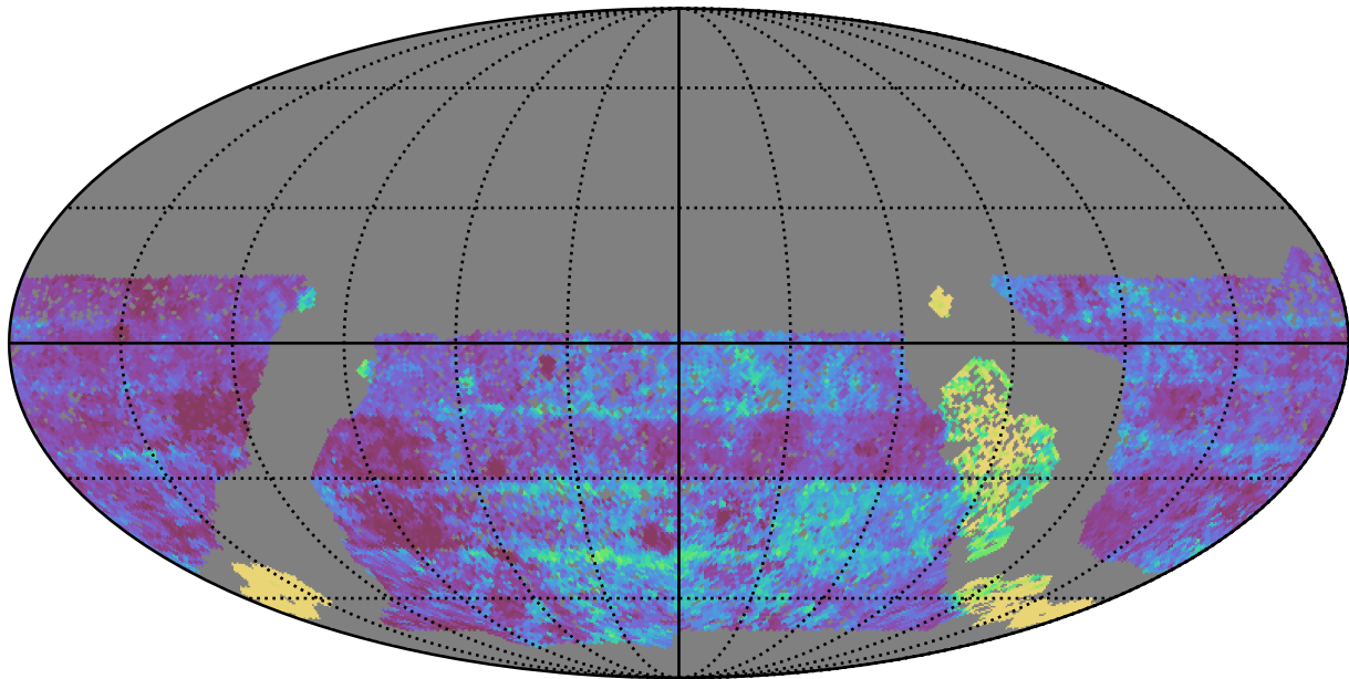
baseline_v3.0_10yrs WFD y band: Median Inter-Night Gap
