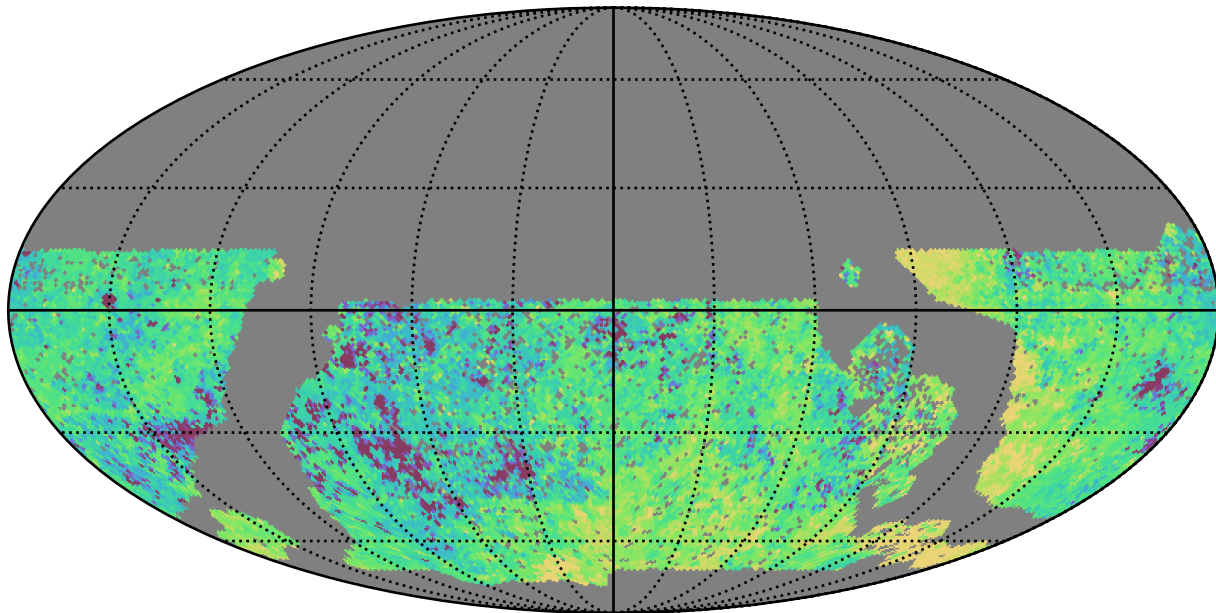
baseline_v3.0_10yrs WFD u band: Median Inter-Night Gap
