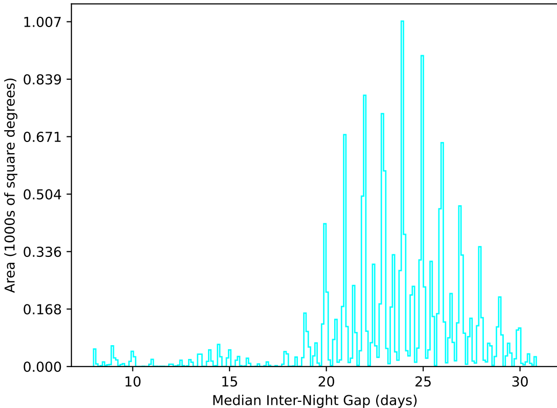
baseline_v3.0_10yrs WFD u band: Median Inter-Night Gap
