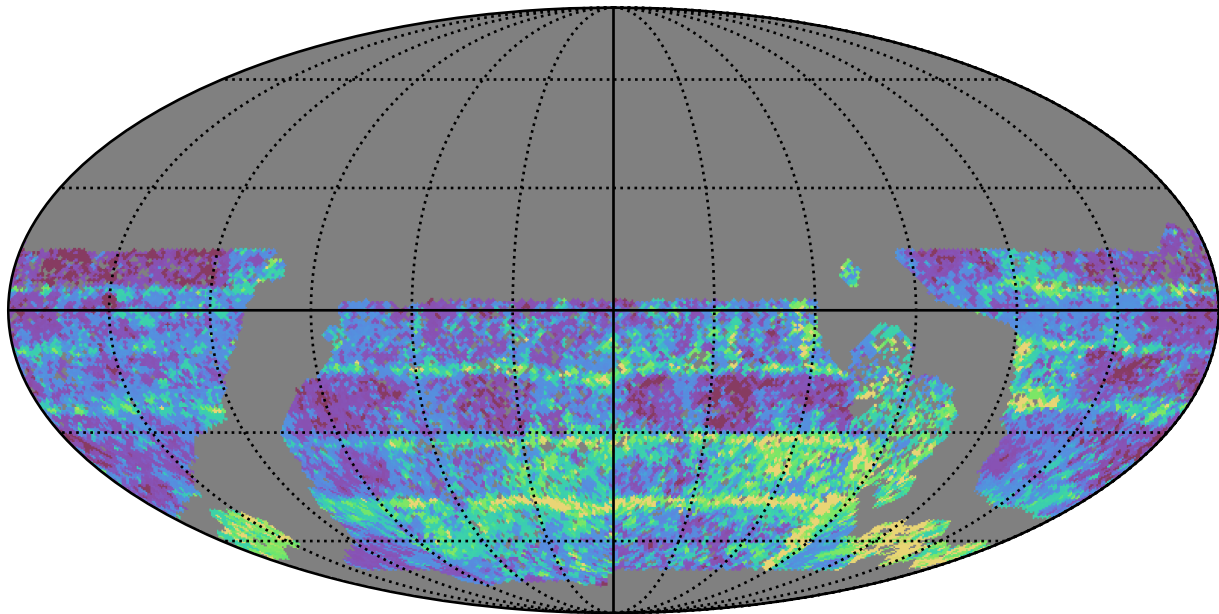
baseline_v3.0_10yrs WFD r band: Median Inter-Night Gap
