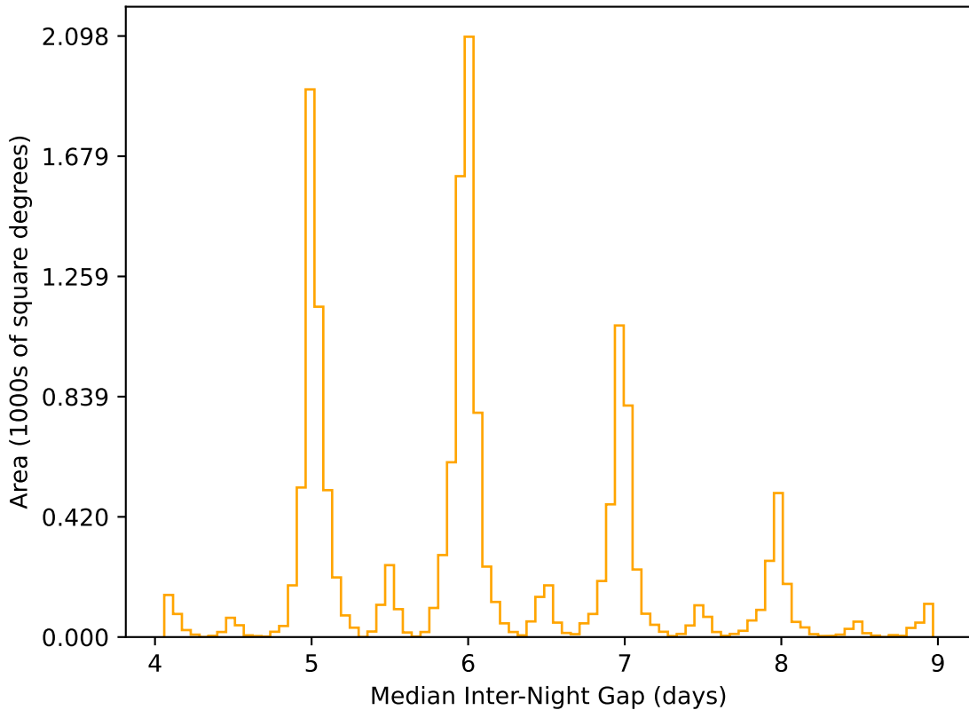
baseline_v3.0_10yrs WFD r band: Median Inter-Night Gap
