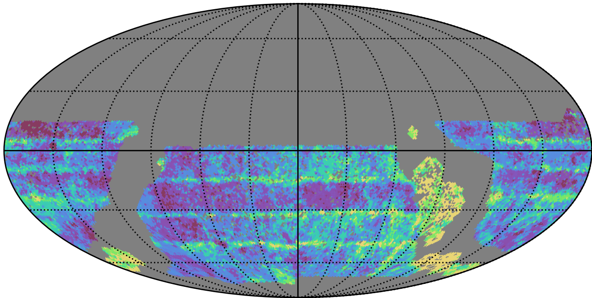
baseline_v3.0_10yrs WFD i band: Median Inter-Night Gap
