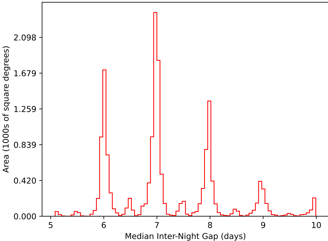
baseline_v3.0_10yrs WFD i band: Median Inter-Night Gap
