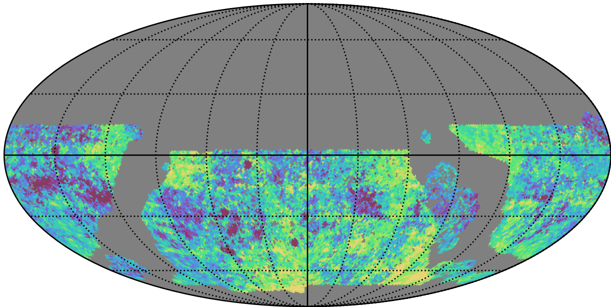
baseline_v3.0_10yrs WFD g band: Median Inter-Night Gap
