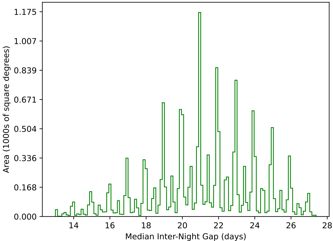
baseline_v3.0_10yrs WFD g band: Median Inter-Night Gap
