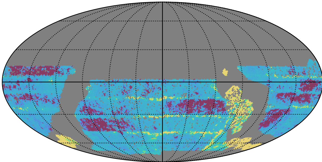
baseline_v3.0_10yrs WFD all bands: Median Inter-Night Gap
