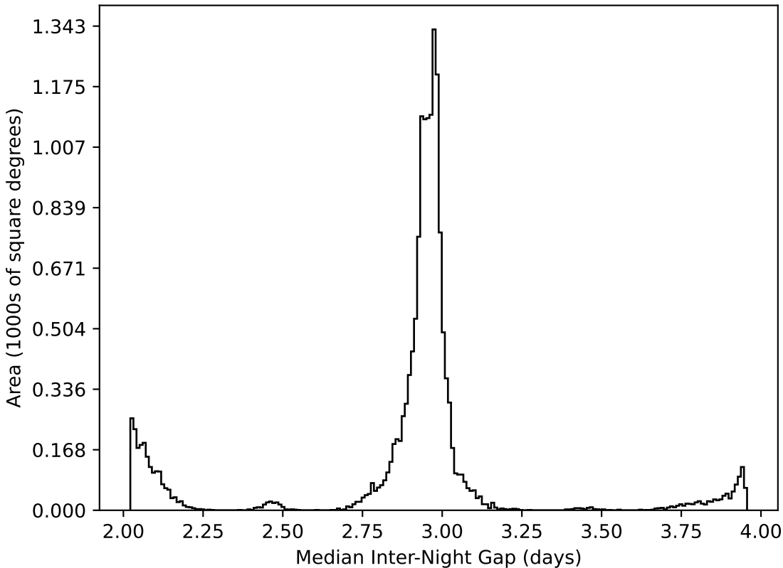
baseline_v3.0_10yrs WFD all bands: Median Inter-Night Gap
