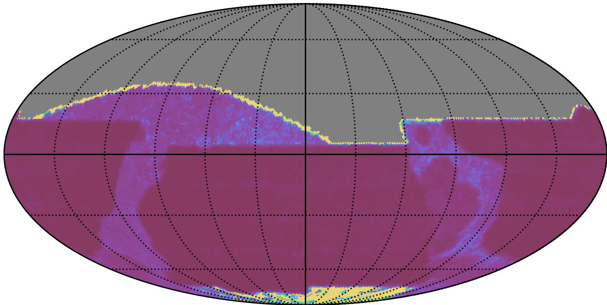
baseline_v3.0_10yrs All sky z band: Median Inter-Night Gap
