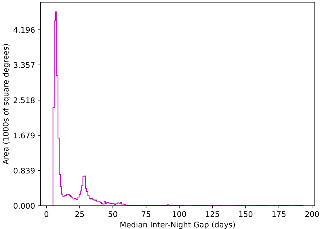
baseline_v3.0_10yrs All sky z band: Median Inter-Night Gap
