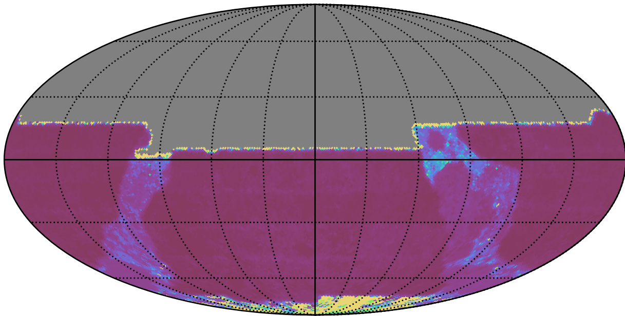
baseline_v3.0_10yrs All sky y band: Median Inter-Night Gap
