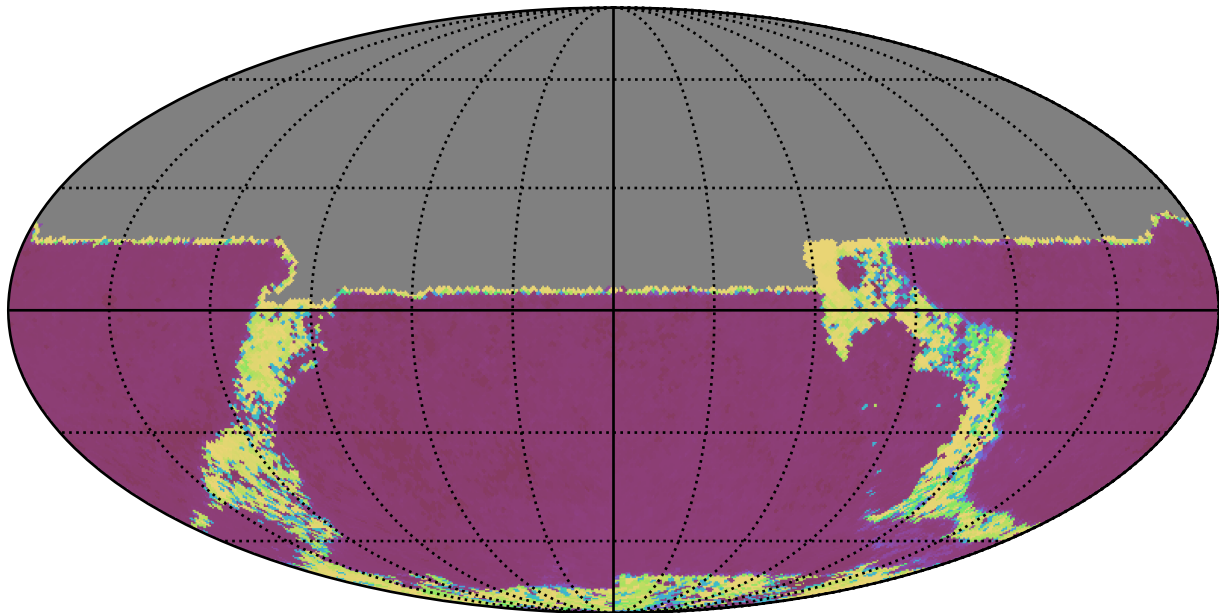
baseline_v3.0_10yrs All sky u band: Median Inter-Night Gap
