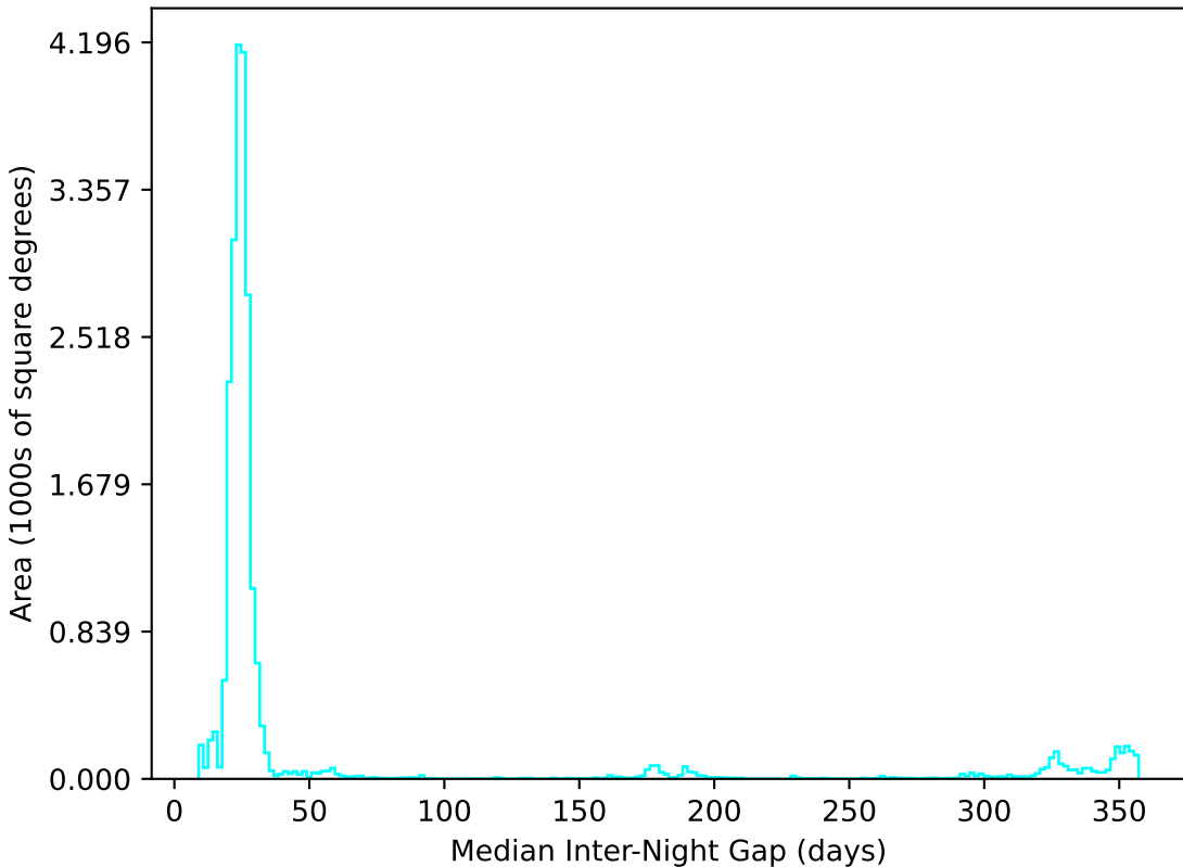
baseline_v3.0_10yrs All sky u band: Median Inter-Night Gap
