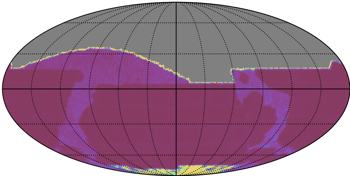
baseline_v3.0_10yrs All sky r band: Median Inter-Night Gap
