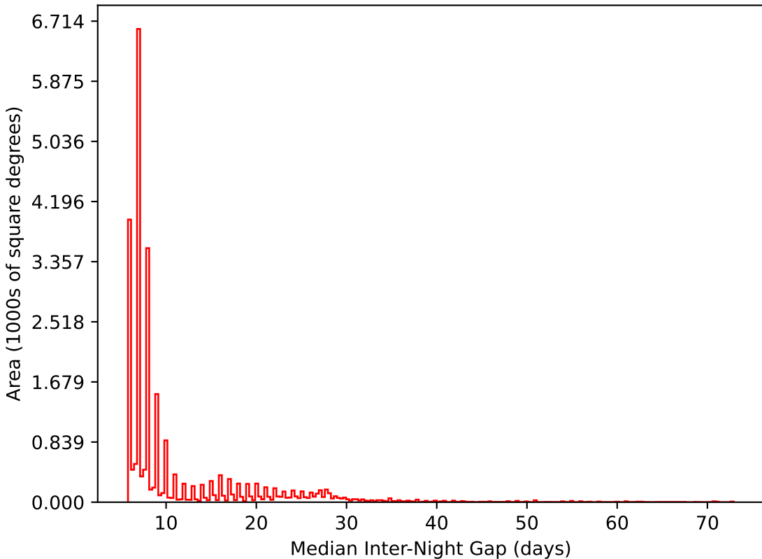
baseline_v3.0_10yrs All sky i band: Median Inter-Night Gap
