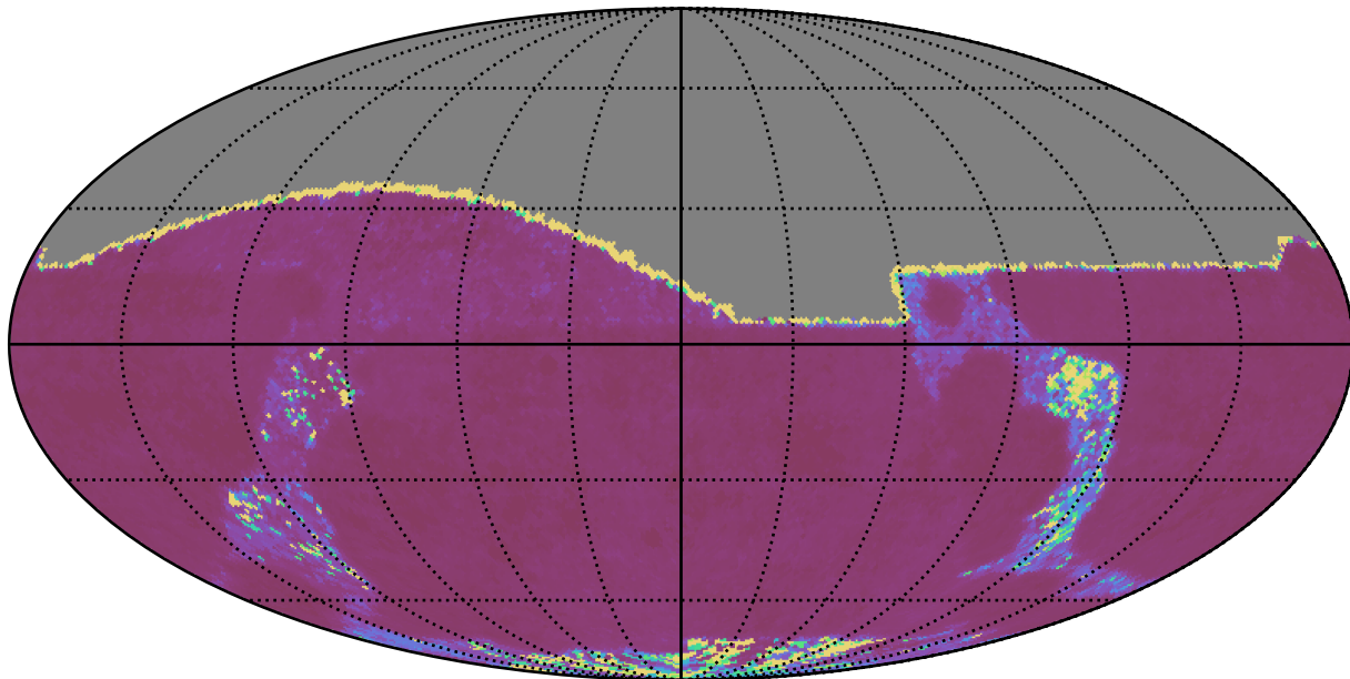
baseline_v3.0_10yrs All sky g band: Median Inter-Night Gap
