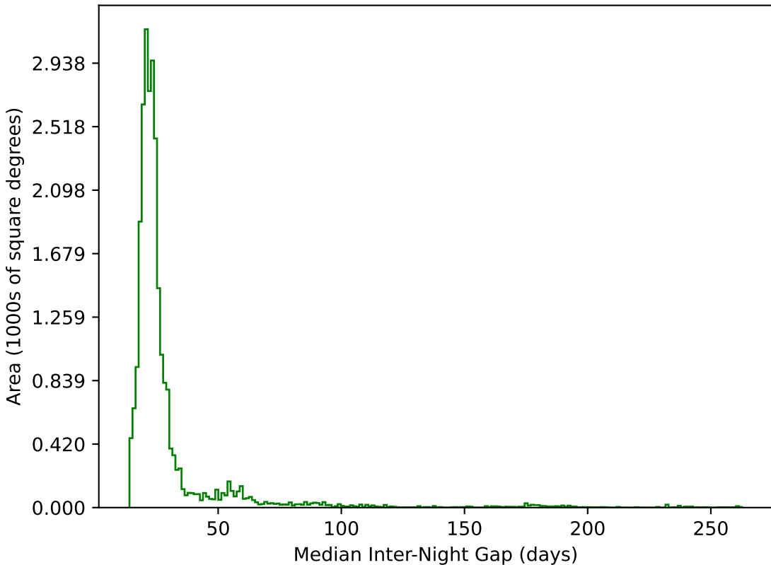
baseline_v3.0_10yrs All sky g band: Median Inter-Night Gap
