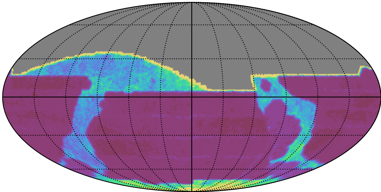
baseline_v3.0_10yrs All sky all bands: Median Inter-Night Gap
