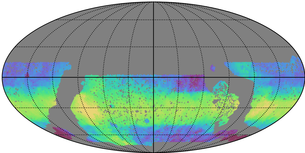
baseline_v3.0_10yrs WFD z band: Median HA
