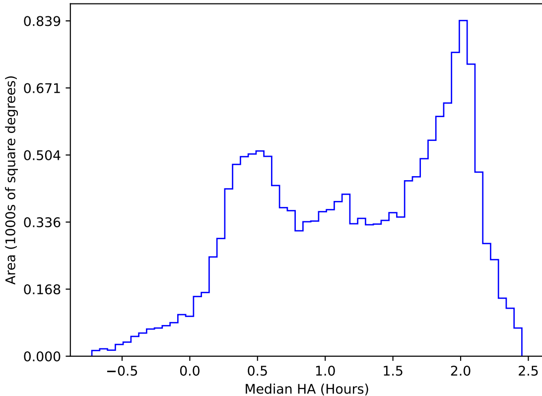
baseline_v3.0_10yrs WFD z band: Median HA
