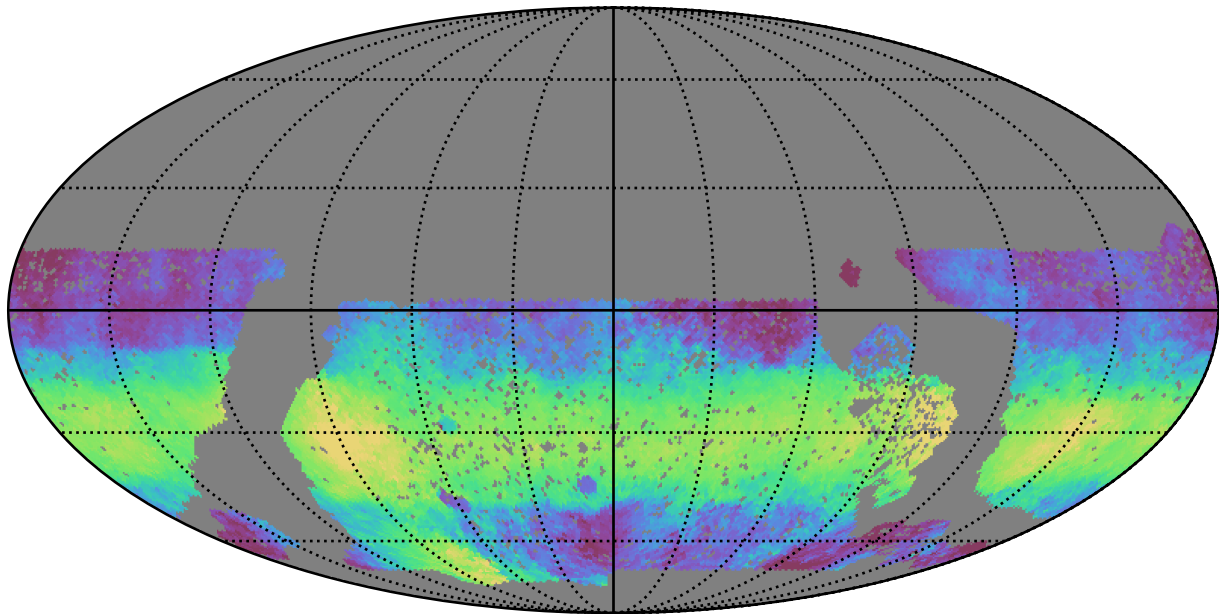
baseline_v3.0_10yrs WFD y band: Median HA
