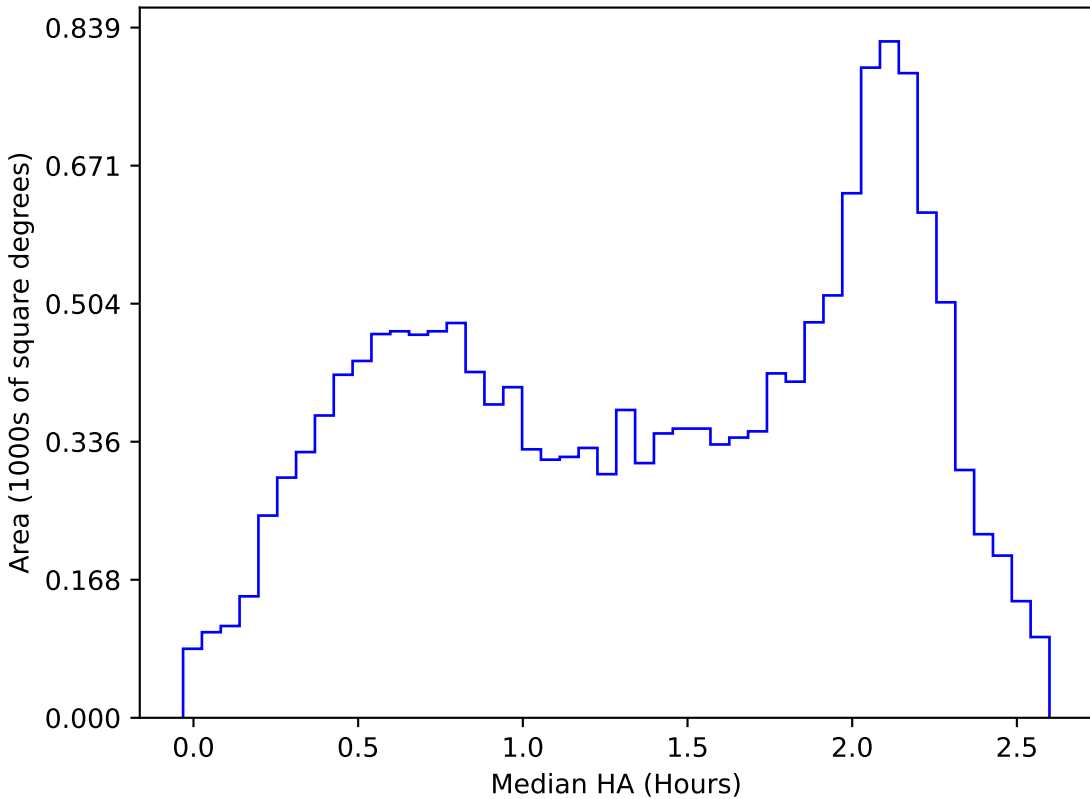
baseline_v3.0_10yrs WFD y band: Median HA
