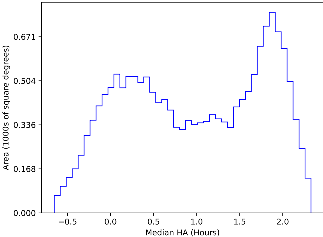
baseline_v3.0_10yrs WFD u band: Median HA
