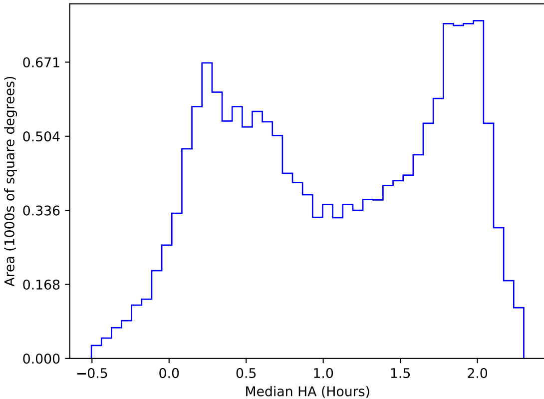
baseline_v3.0_10yrs WFD r band: Median HA
