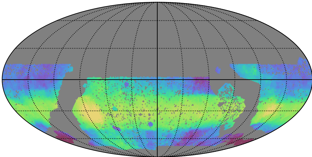
baseline_v3.0_10yrs WFD i band: Median HA
