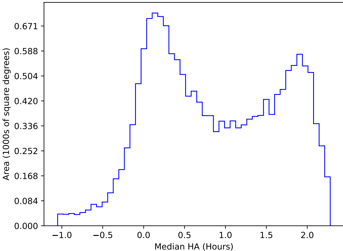
baseline_v3.0_10yrs WFD g band: Median HA
