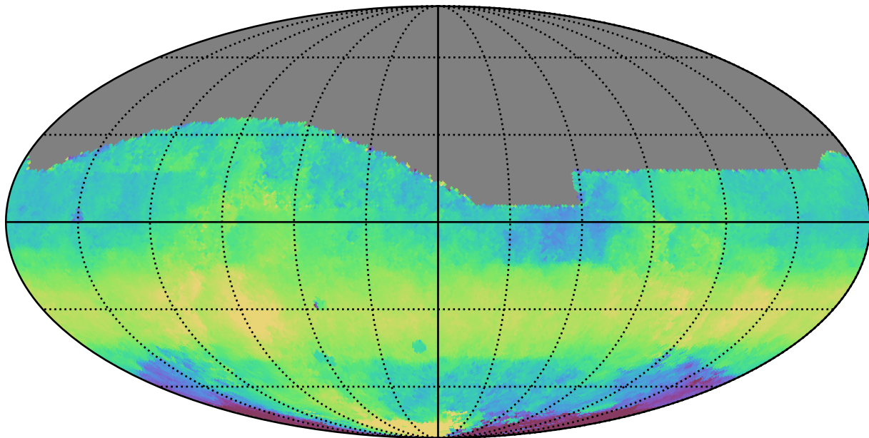
baseline_v3.0_10yrs All sky z band: Median HA
