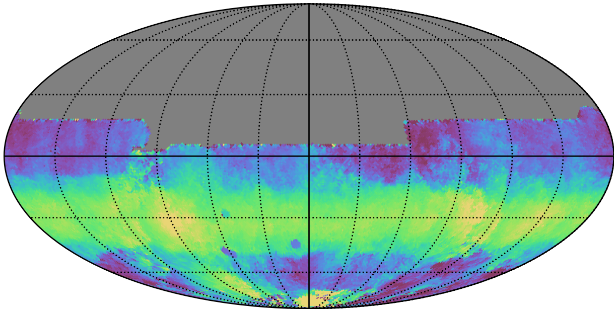
baseline_v3.0_10yrs All sky y band: Median HA
