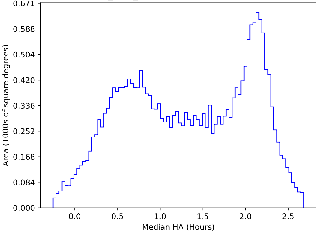
baseline_v3.0_10yrs All sky y band: Median HA
