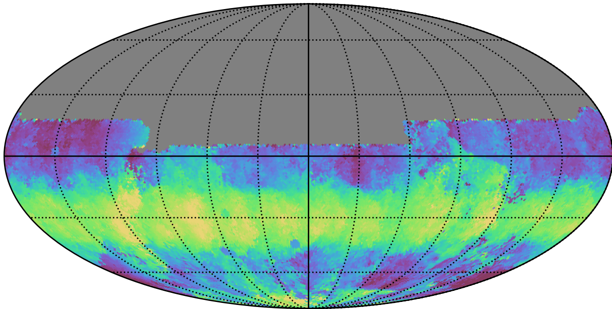
baseline_v3.0_10yrs All sky u band: Median HA
