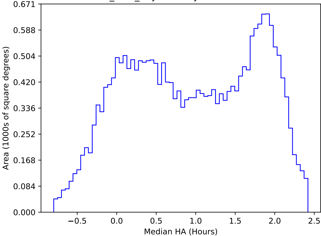
baseline_v3.0_10yrs All sky u band: Median HA
