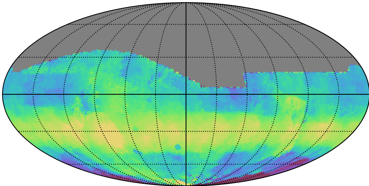
baseline_v3.0_10yrs All sky r band: Median HA
