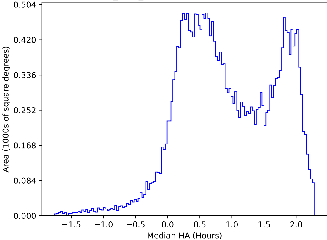
baseline_v3.0_10yrs All sky r band: Median HA
