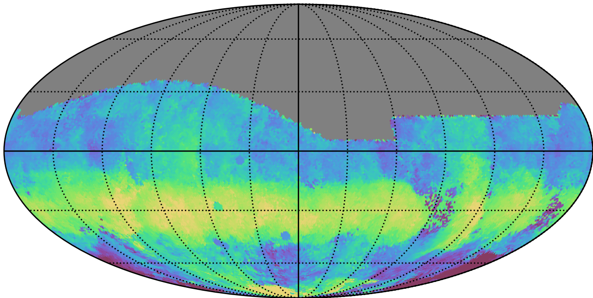
baseline_v3.0_10yrs All sky g band: Median HA
