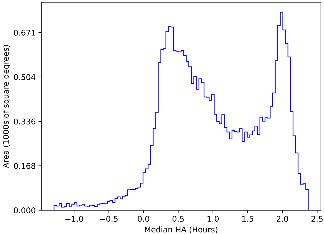
baseline_v3.0_10yrs All sky all bands: Median HA
