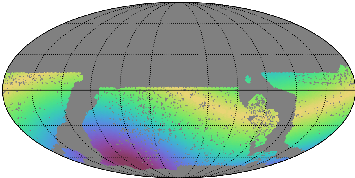
baseline_v3.0_10yrs WFD z band: Max solarElong
