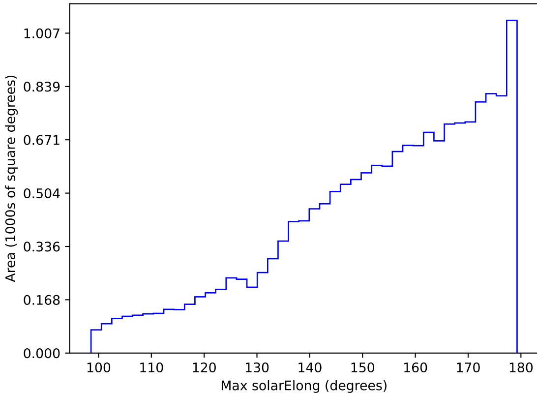
baseline_v3.0_10yrs WFD z band: Max solarElong
